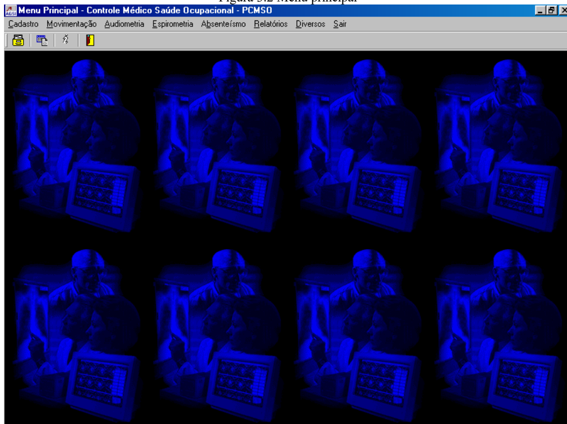
Figura 3.2 Menu principal
